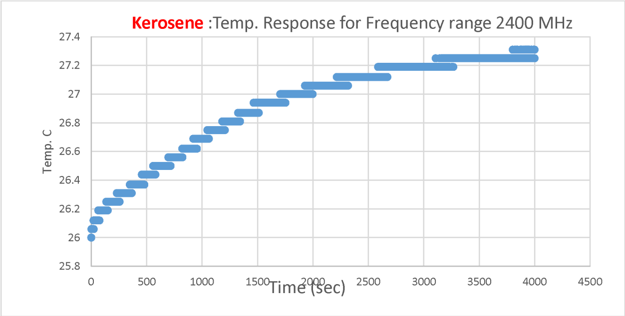
Graph 1.28—Relationship Between Temperature Measurements and Radiation Frequency at 2400 Mhz for Kerosene
