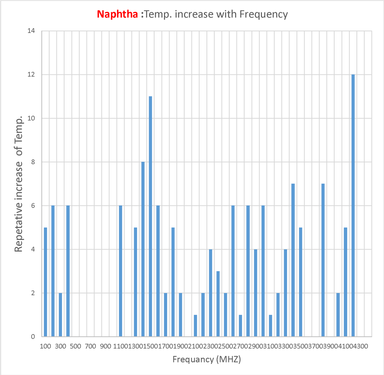
Graph 1.18—Relationship Between Frequency and Temperature Rise Repetition for Naphtha.
