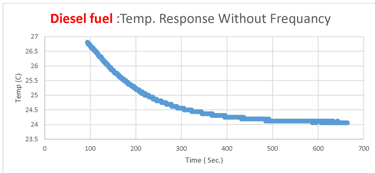
Graph 1.35—Relationship Between Temperature Measurements and Time without radiation for Diesel Fuel.
