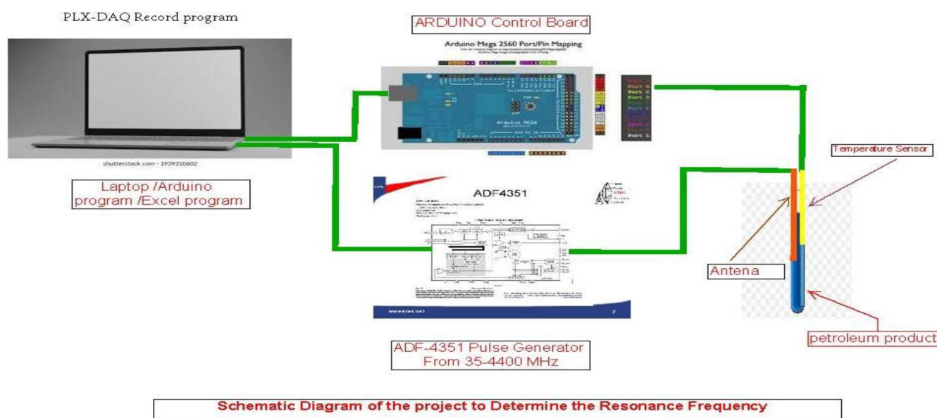
Fig. 1.6—The Research system for generate pulse, record and Analysis.
